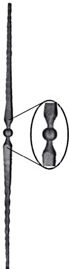
H.950mm □20->14mm PAF 15
